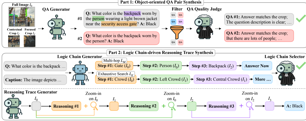
Figure 3: A detailed overview of LOGT SFT data synthesis engine. Part 1 (top; Section 3.1) synthesizes visual search QA pairs using the full image ( I_0 ) along with rich visual contexts ( I_C and I_F , top left) related to randomly selected target objects. After generating candidate QAs, we apply a simple heuristic filter and use a VLM-as-a-Judge to ensure quality. Part 2 (bottom; Section 3.2) generates reasoning traces for the selected QA. For easy questions, we directly generate traces without tool calls (omitted here). For other questions, we first create logic chains ( L_M and L_E ) based on two human-like strategies. A logic chain selector then chooses the more appropriate one, which is subsequently used to guide the synthesis of multi-turn reasoning traces with tool use.
