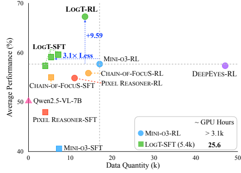
Figure 2: Result highlights. By applying SFT to a Qwen2.5-VL-7B model using 5.4k to 7.1k of our synthesized data, LOGT-SFT surpasses the best-performing MINI-O3-RL on average across seven test sets, while using up to 3.1× less data and >120× fewer GPU hours. With a simple RL setup without any tool-specific design, LOGT-RL further outperforms baselines by 9.59.
