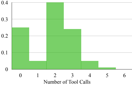
Figure 10: Normalized distribution of ZOOM-IN call counts in the SFT dataset generated by LOGT. The number of tool calls per trace in the dataset ranges from 0 (direct answering without tool use) to 6.
