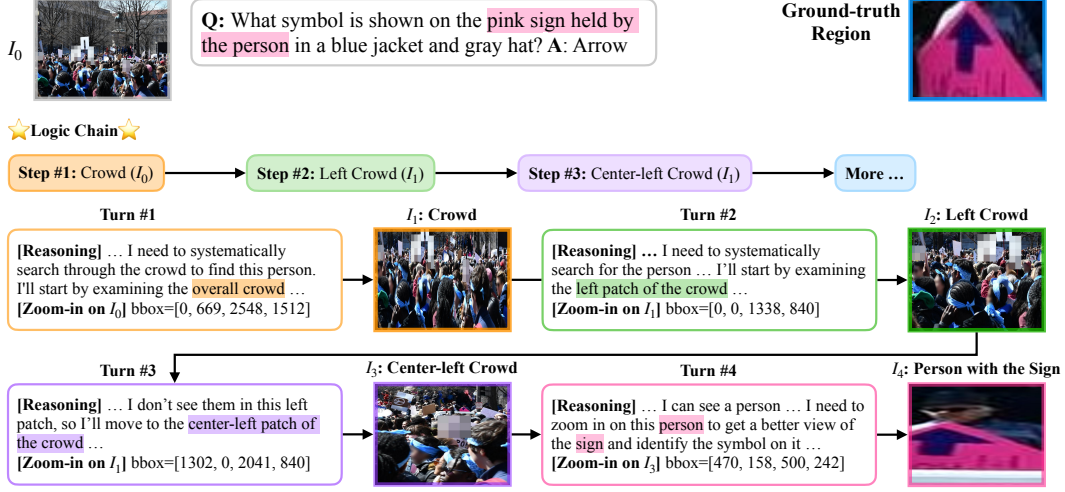
Figure 9: An example of an exhaustive search logic chain and its corresponding tool-use reasoning trace. To locate the pink sign held by a person in the crowd, the logic chain begins by instructing the trace generator (see Section 3.2) to identify the crowd, then systematically search it from left to right. Since the trace generator successfully detects the target sign and the person in the crop returned by the third ZOOM-IN call, it stops scanning the rest of the crowd and instead zooms in on the identified region to extract the final answer.
