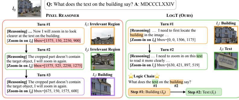
(a) PIXEL REASONER vs. LOGT. The example trace in PIXEL REASONER SFT data randomly introduces errors when synthesizing multi-turn tool calls, and the erroneous bounding boxes are highlighted in red. In contrast, ours follows a coherent logic chain: first locating the building, and then locating the text.
