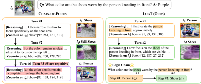
(b) CHAIN-OF-FOCUS vs. LOGT. The example trace in CHAIN-OF-FOCUS SFT data repeatedly zooms in on the shoes over six turns, despite correctly identifying the target region in the first turn. This redundant reasoning, highlighted in red, reflects tool call inefficiency. In contrast, LOGT demonstrates a coherent reasoning chain: first locating the person, then progressively narrowing down to the shoes.
