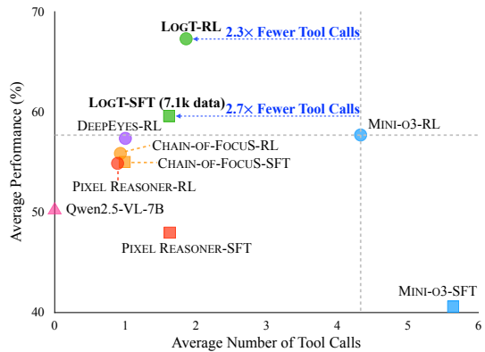
Figure 6: Tool call efficiency. We report the average number of tool calls per question across the seven test sets. Despite achieving better performance compared to prior SOTA, LOGT-SFT model uses 2.7\times fewer tool calls, and LOGT-RL uses 2.3\times fewer.
