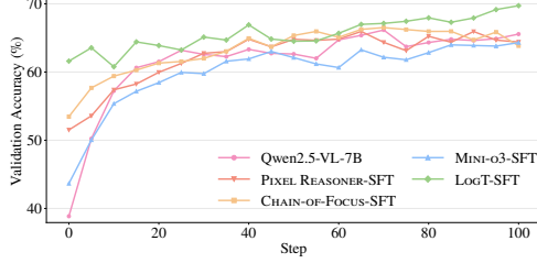
Figure 4: Training dynamics after applying our simple RL procedure to the baselines and LOGT-SFT. During RL, our model’s validation accuracy steadily improves, whereas other SFT baselines perform on par with, or worse than zero-RL. LOGT greatly improves the RL performance ceiling.
