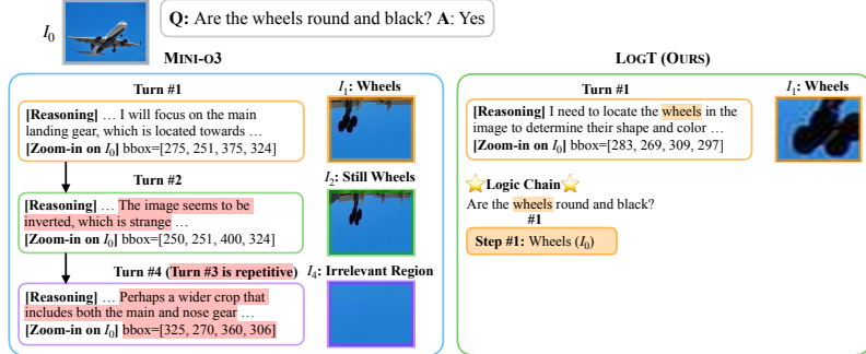
(c) MINI-O3 vs. LOGT. The example trace in MINI-O3 SFT data correctly finds the wheels in the first turn but mistakenly claims that the crop returned by ZOOM-IN is inverted, leading to two redundant ZOOM-IN calls. Ultimately, it zooms in on an entirely irrelevant region. The redundant reasoning and the incorrect ZOOM-IN call are highlighted in red. In contrast, LOGT makes a single ZOOM-IN call to locate the wheels and then directly reaches the correct answer.
