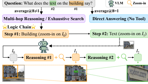
Figure 1: Main idea. We generate reasoning traces based on human-like strategies including (i) direct answering for simple questions, (ii) multi-hop reasoning by focusing on different regions, and (iii) exhaustive search for more difficult cases. For easy questions where the base model’s average@8 is 1, we synthesize direct answering traces without ZOOM-IN. Otherwise, we first generate logic chains that specify key tool-use steps and then use them to guide the VLM in synthesizing tool-use reasoning traces.
