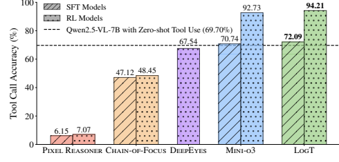
Figure 5: Tool call accuracy. We report tool call accuracy on V^* for the base model and all post-trained models. The base model is prompted to use ZOOM-IN in a zero-shot setting. Our LOGT-SFT and LOGT-RL models achieve the highest ZOOM-IN accuracy.
